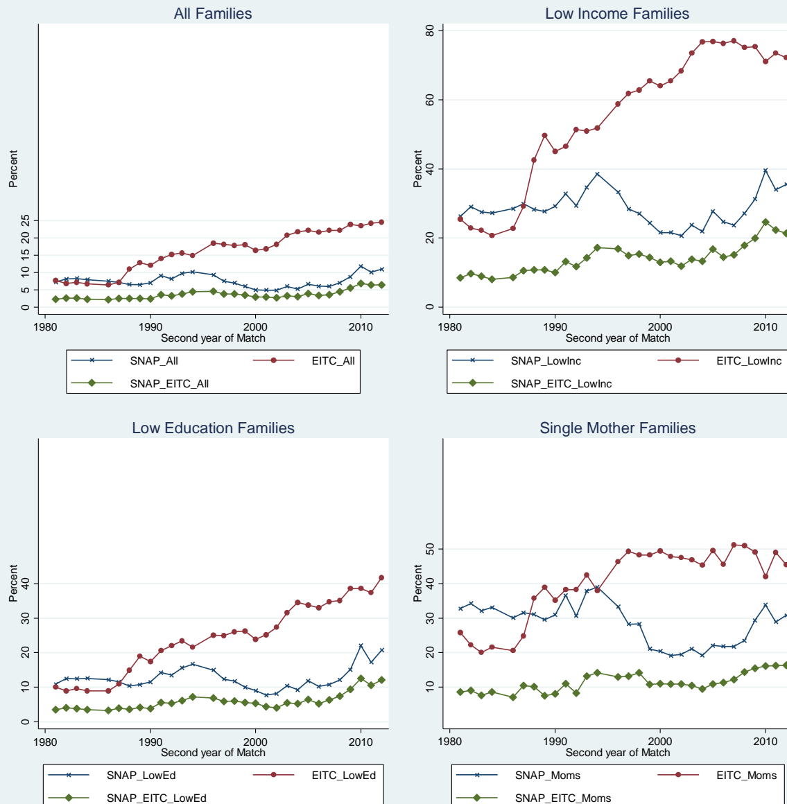
Figure 1. Trends in Two-Year SNAP and EITC/CTC Participation
