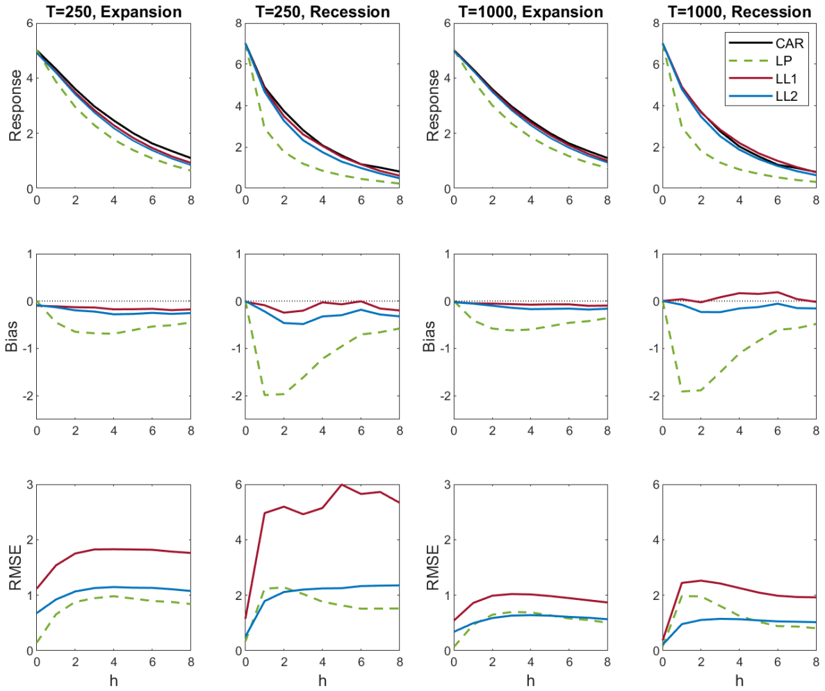
Figure 5: State Dependent Model, \delta = 2
